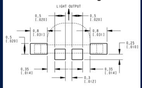
Recommended Soldering Pattern For Reflow Soldering
