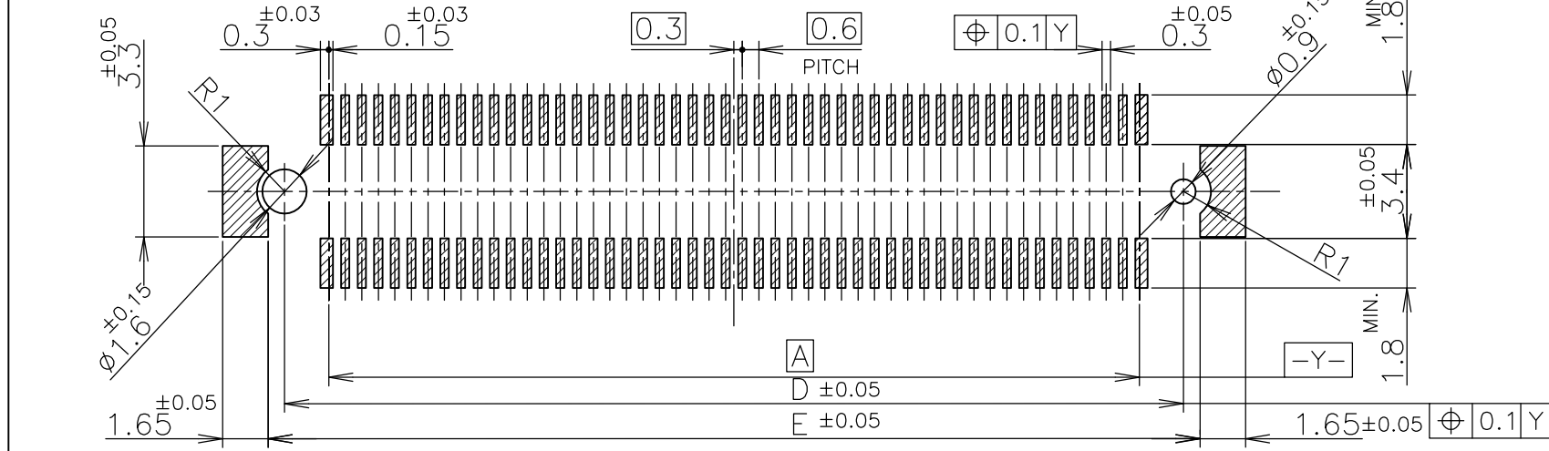
REFERENCE P.C.BOARD LAYOUT
