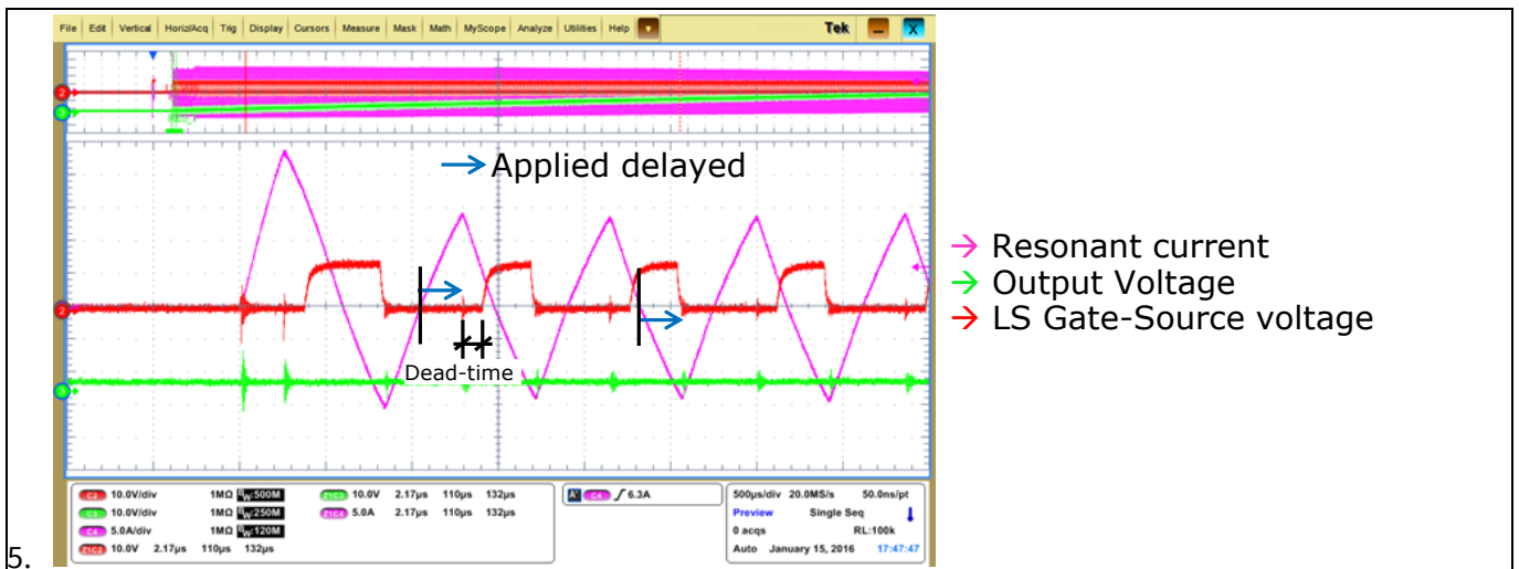
5. Figure 27 LS-HS driving signal change is applied with a delay after the resonant current crosses zero to guarrante current polarity change and avoid hard-conmuation.
