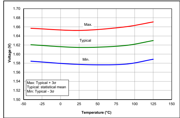
FIGURE 29-57: POR Release Voltage.
