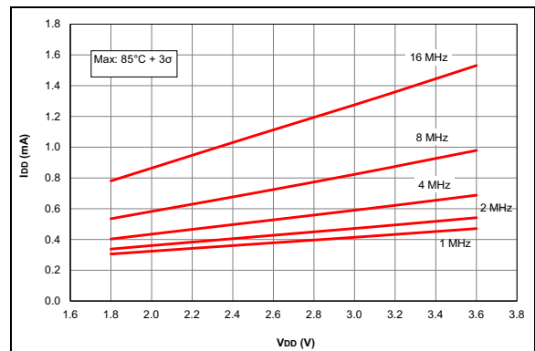
FIGURE 29-18: I_{DD} Maximum, HFINTOSC Mode, PIC12LF1612/16F1613 Only.
