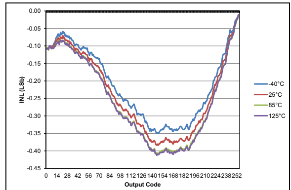
FIGURE 29-93: Typical DAC INL Error, V_{DD} = 5.0V , V_{REF} = \text{External } 5V , PIC12F1612/16F1613 Only.
