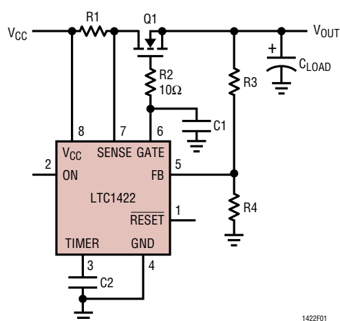
Figure 1. Supply Control Circuitry
