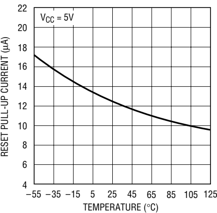
RESET Pull-Up Current vs Temperature
