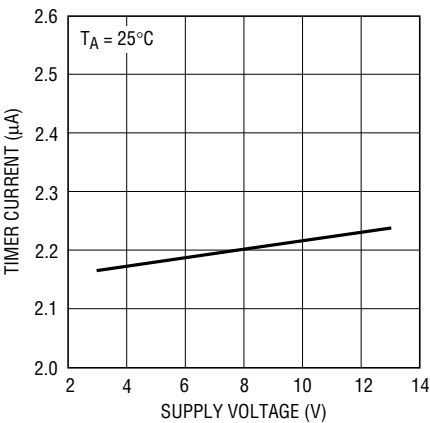
TIMER Current vs Supply Voltage
