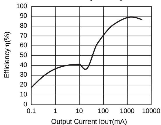
R1224N332G ( V_{IN}=10V )
