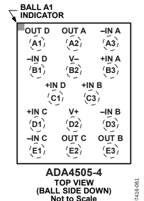
Figure 6. 14-Ball WLCSP (CB-14-1)
