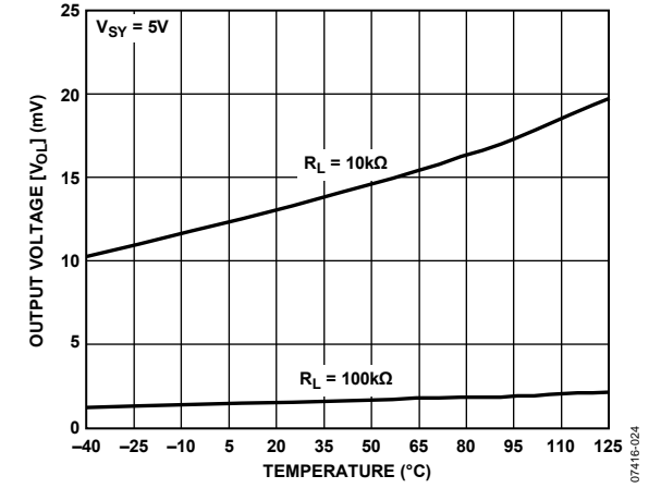
Figure 24. Output Voltage ( V_{O} ) vs. Temperature
