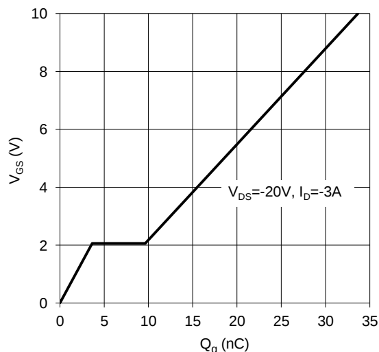
Figure 12. Gate Charge
