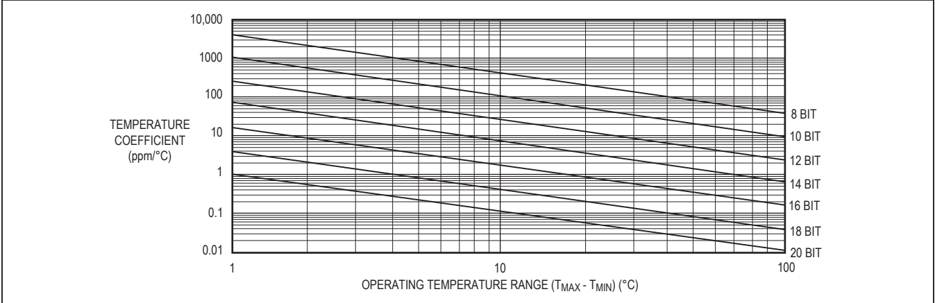
Figure 4. Temperature Coefficient vs. Operating Temperature Range for a 1 LSB Maximum Error
