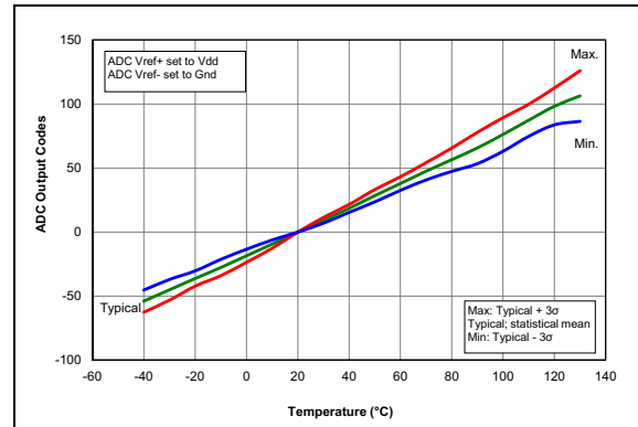
FIGURE 31-104: Temp. Indicator Slope Normalized to 20°C, Low Range, V_{DD} = 3.0V , PIC16F1784/6/7 Only.
