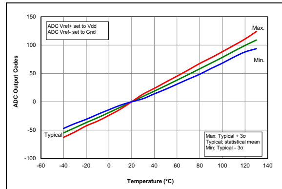
FIGURE 31-106: Temp. Indicator Slope Normalized to 20°C, Low Range, V_{DD} = 3.0V , PIC16LF1784/6/7 Only.
