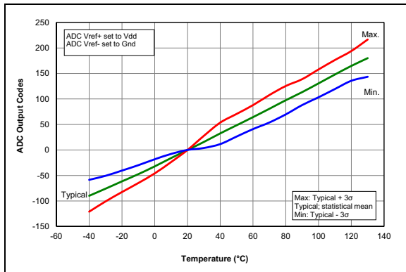
FIGURE 31-105: Temp. Indicator Slope Normalized to 20°C, Low Range, V_{DD} = 1.8V , PIC16LF1784/6/7 Only.
