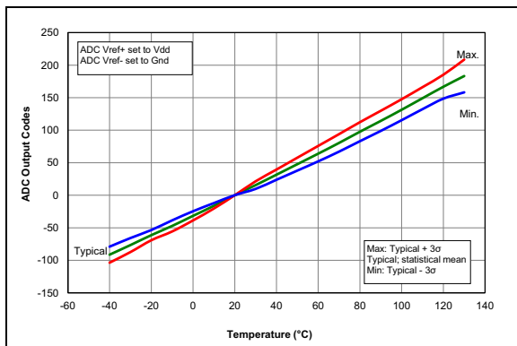
FIGURE 31-107: Temp. Indicator Slope Normalized to 20°C, High Range, V_{DD} = 3.6V , PIC16LF1784/6/7 Only.
