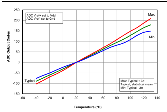
FIGURE 31-103: Temp. Indicator Slope Normalized to 20°C, High Range, V_{DD} = 3.6V , PIC16F1784/6/7 Only.
