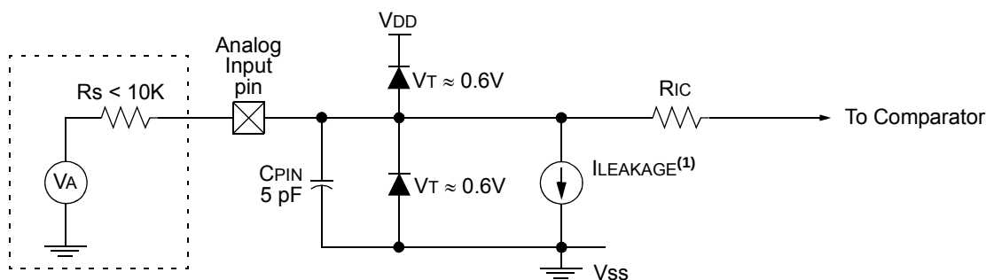
FIGURE 20-4: ANALOG INPUT MODEL
