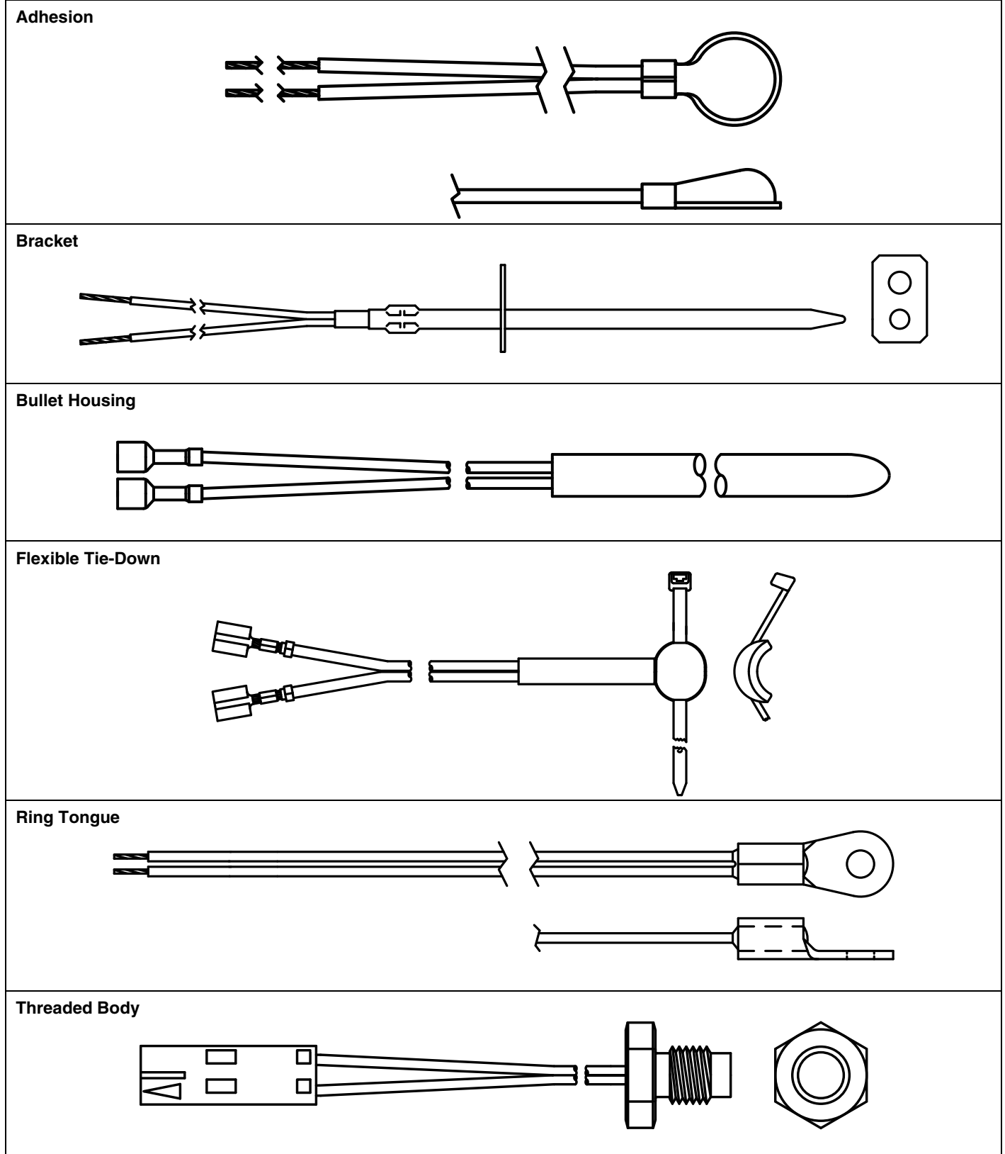
Figure 1. Mounting Methods
