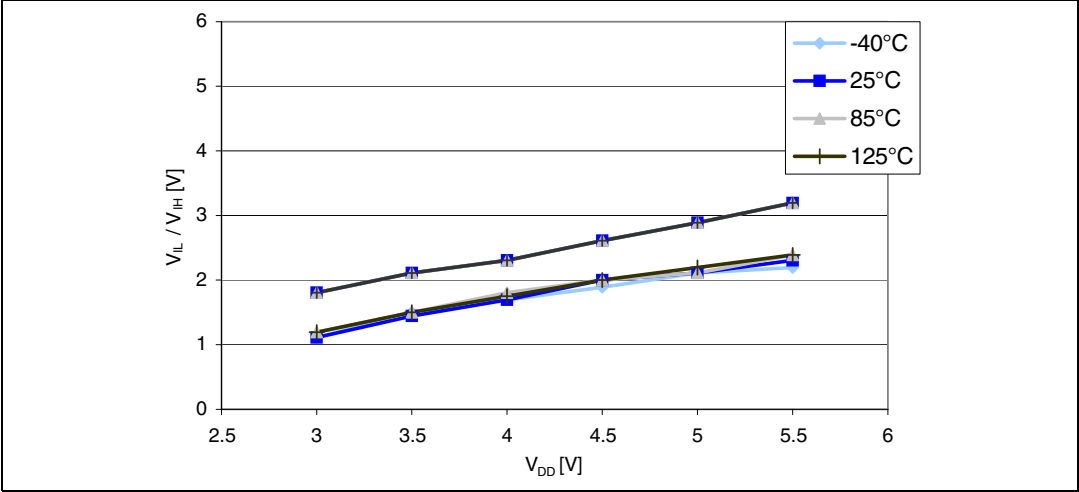
Figure 20. Typical V_{IL} and V_{IH} vs V_{DD} @ four temperatures
