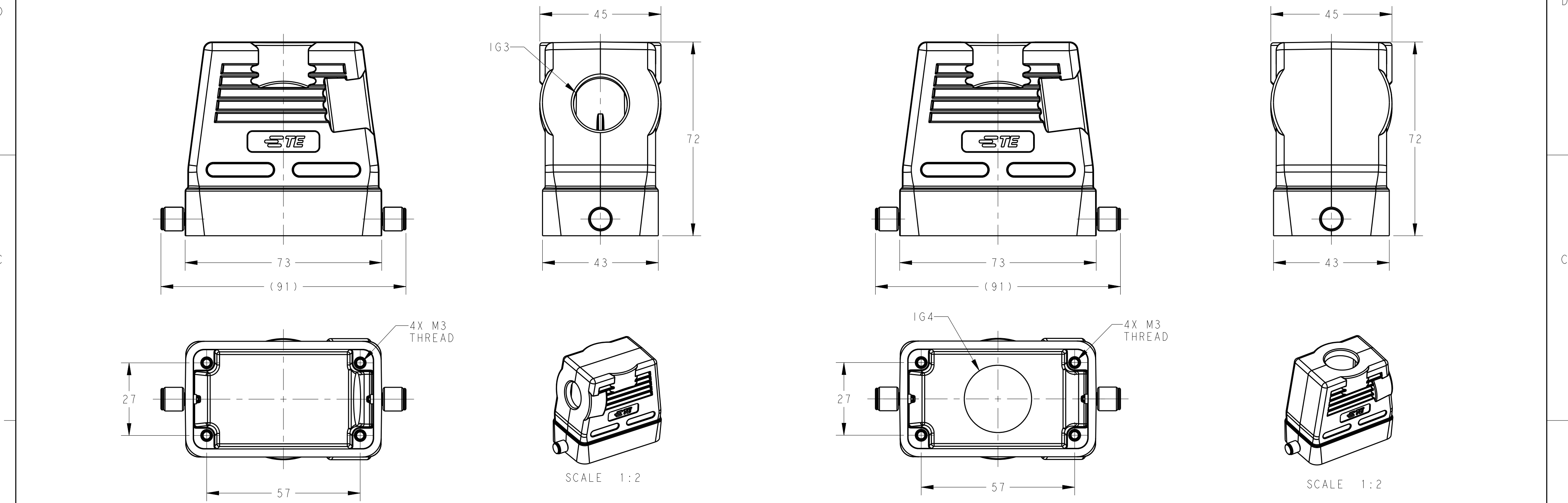
TYPE 3: LOW CONSTRUCTION, SIDE ENTRY TYPE 4: HIGH CONSTRUCTION, TOP ENTRY
