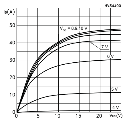
Figure 5. Output characteristics
