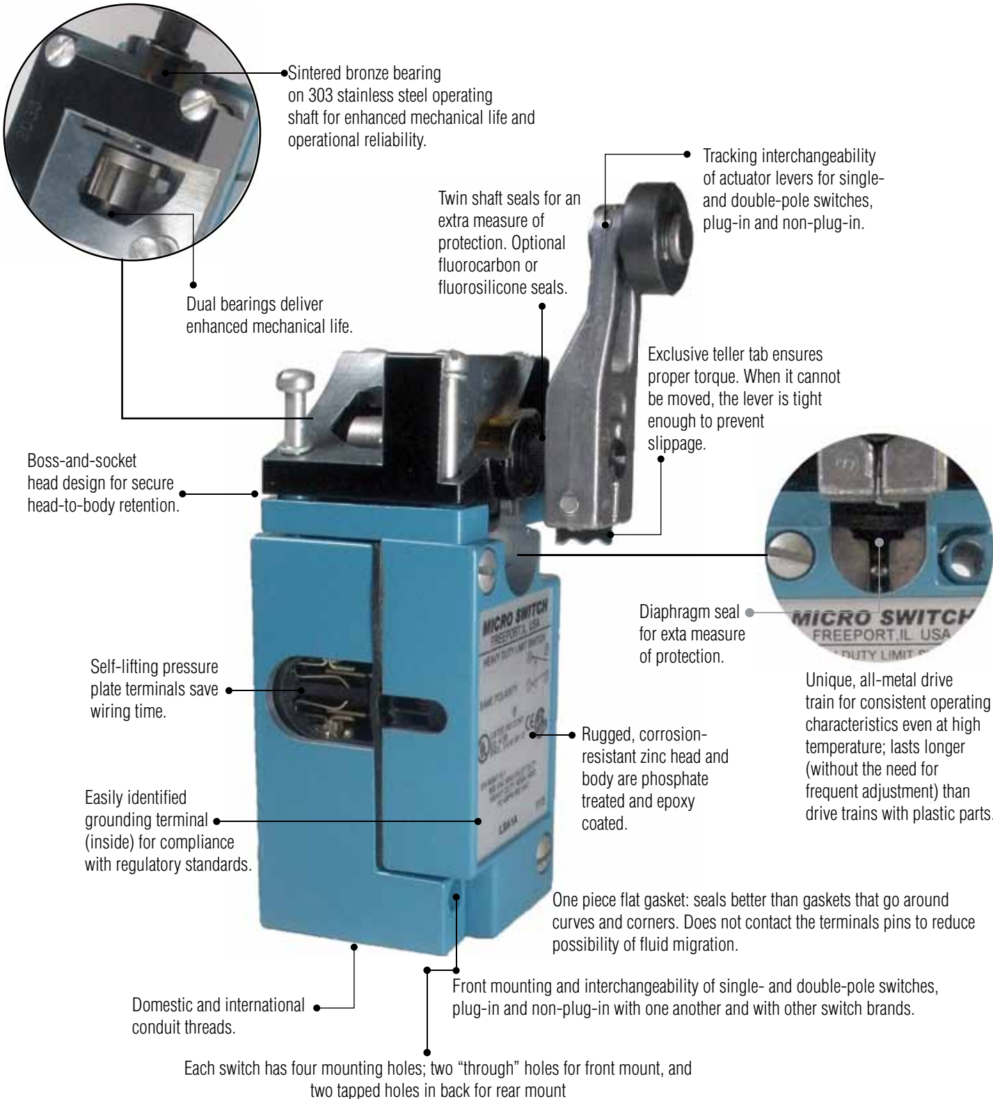
Figure 1. MICRO SWITCH™ HDLS SERIES FEATURES AND OPTIONS
