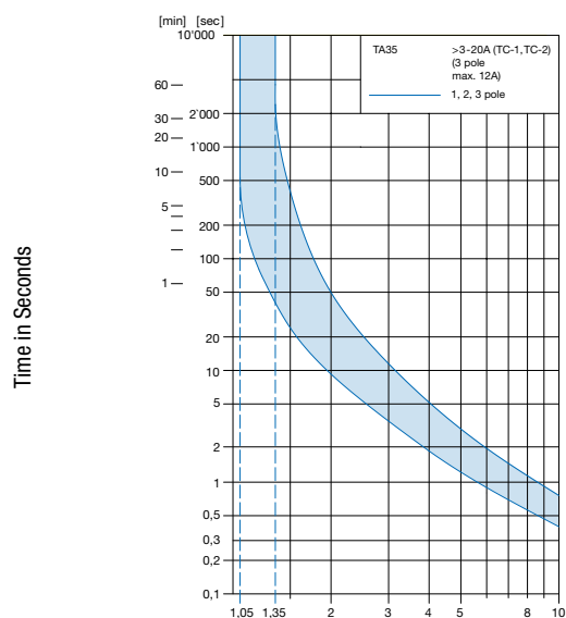
Tripping Characteristics I_n 3\text{ -}20\text{ A}
