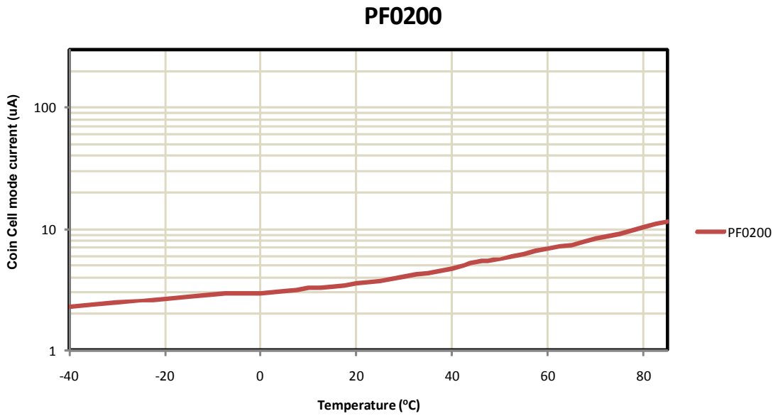
Figure 4. Coin Cell Mode Current Versus Temperature
