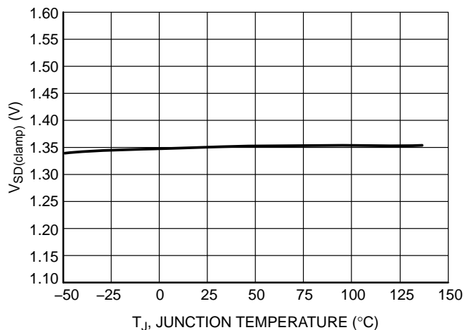
Figure 46. SD Pin Clamp Voltage vs. Temperature
