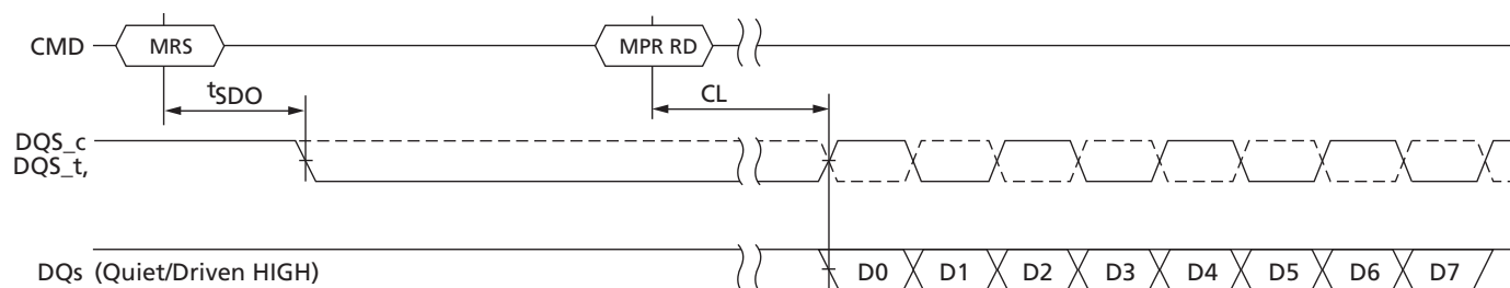
Figure 115: READ Preamble Training
