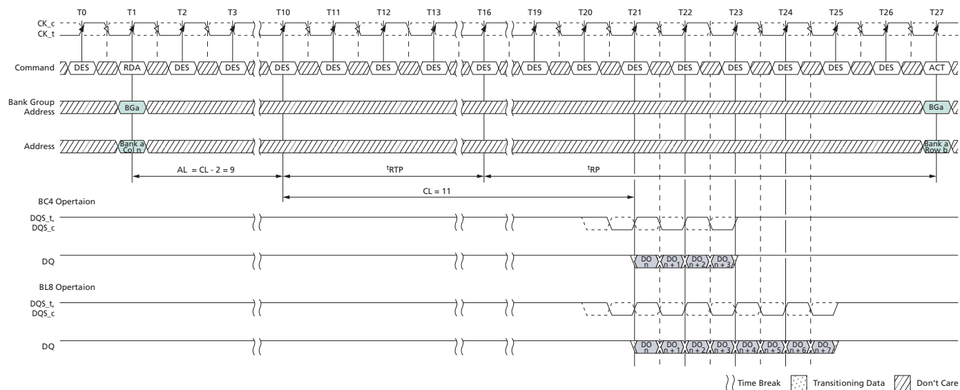
Figure 156: READ with Auto Precharge, Additive Latency, and 1 st CK Preamble
