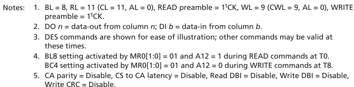
Figure 151: READ (BL8) to WRITE (BC4) OTF with 2 t CK Preamble in Same or Different Bank Group
