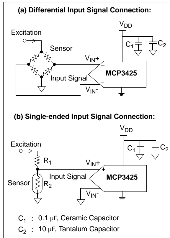
FIGURE 6-4: Differential and Single-Ended Input Connections.
