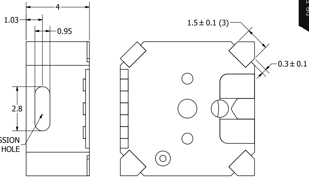
DETAIL "B"
