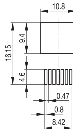
Figure 18 PG-TO263-7-1 (Plastic Green Transistor Single Outline Package)
