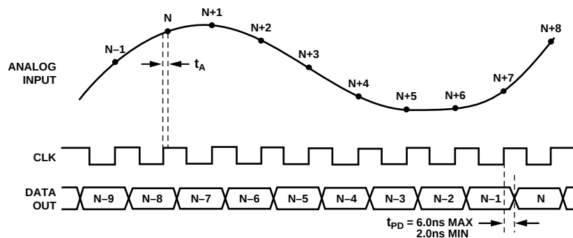
Figure 2. Timing Diagram
