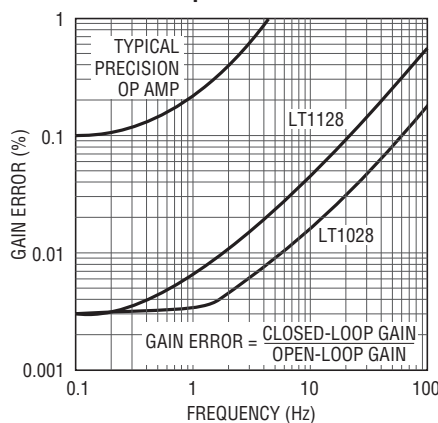
Gain Error vs Frequency
