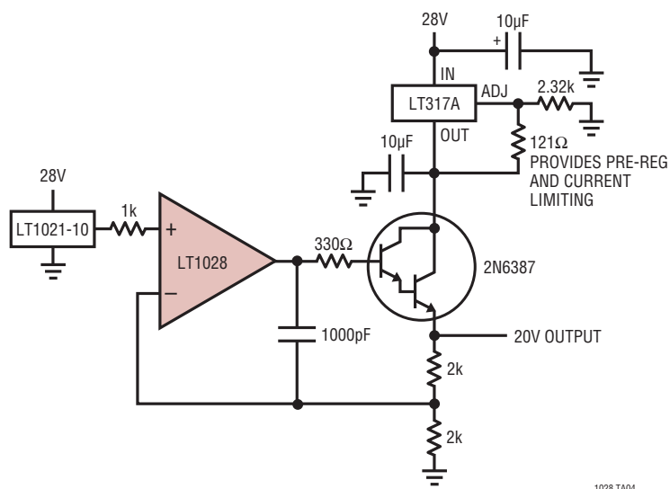
Low Noise Voltage Regulator
