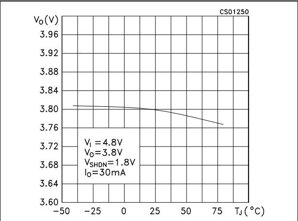
Figure 4. Output voltage vs. temperature ( V_O = 3.8\text{V} )
