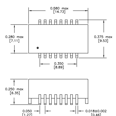
N6 Package
