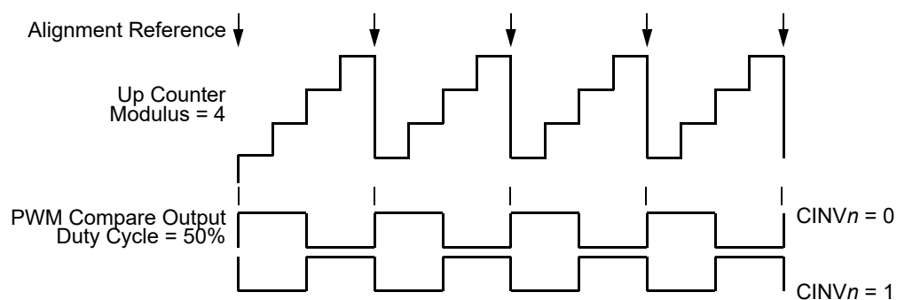
Figure 12-43. Edge-Aligned PWM Output
