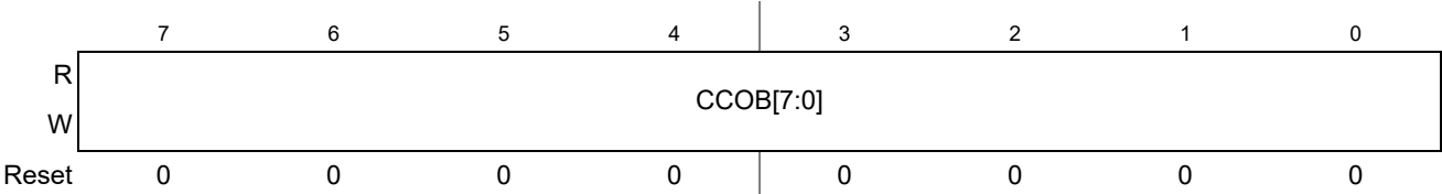
Figure 18-25. Flash Common Command Object 3 Low Register (FCCOB3LO)
