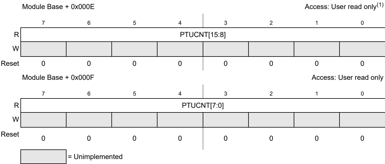
Figure 13-12. PTU Counter Register (PTUCNTH, PTUCNTL)
