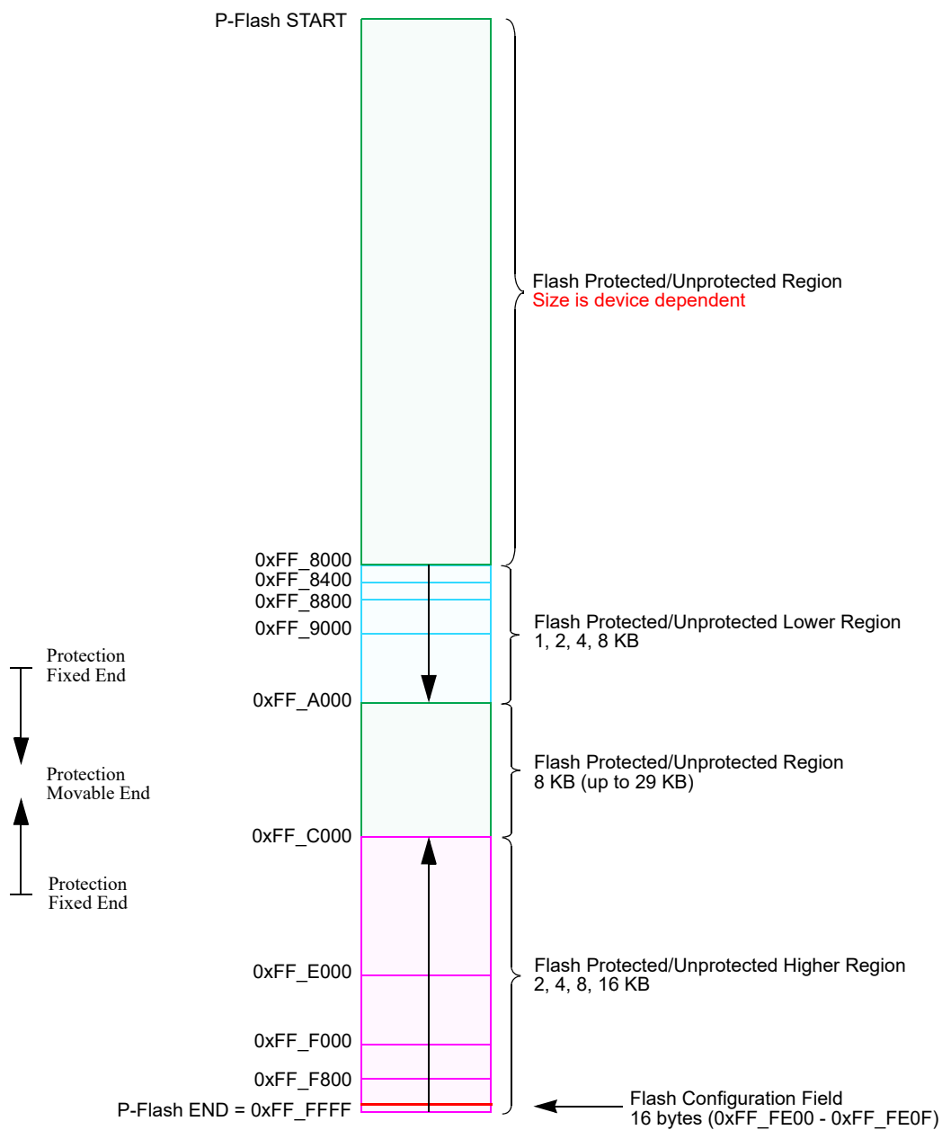
Figure 18-2. P-Flash Memory Map With Protection Alignment
