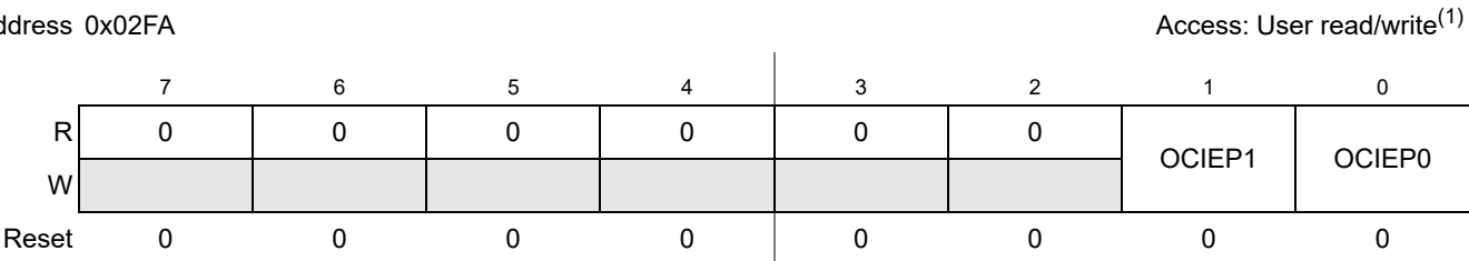
Figure 2-27. Port P Over-Current Interrupt Enable Register
