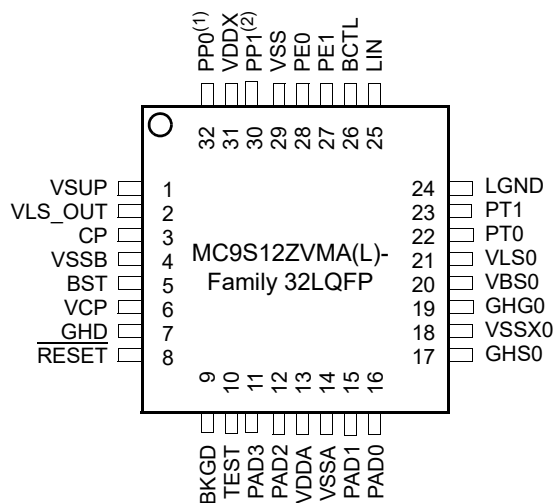
Figure 1-4. MC9S12ZVMA-Family 32-pin LQFP pin out
