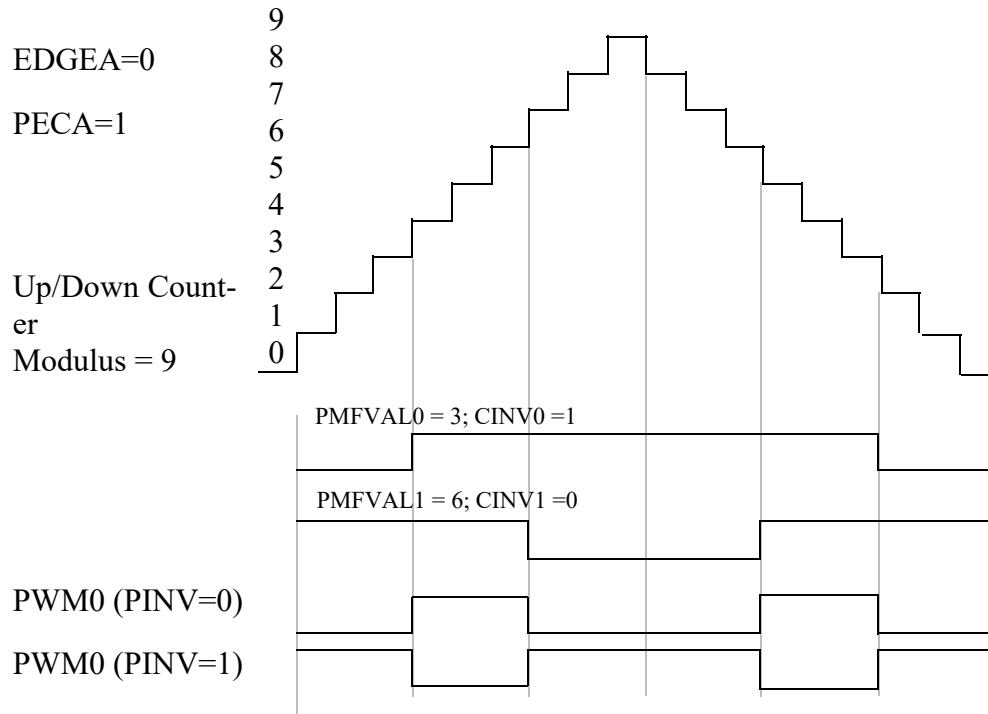
Figure 12-65. Double-Switching PWM Output VAL0&lt;VAL1 (Center-Aligned)
