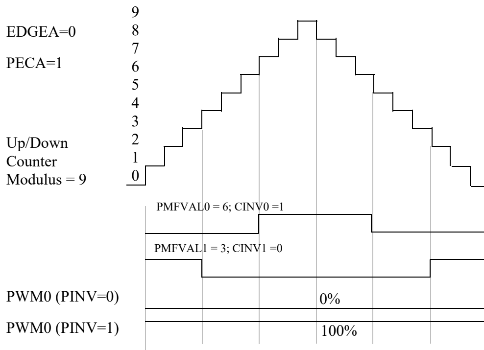
Figure 12-66. Double-Switching PWM Output VAL0&gt;VAL1 (Center-Aligned)
