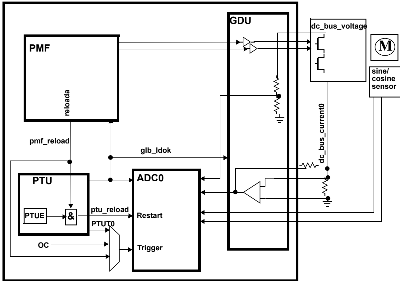
Figure 1-5. Motor Control Module interfaces
