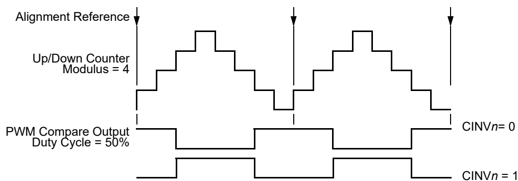
Figure 12-42. Center-Aligned PWM Output
