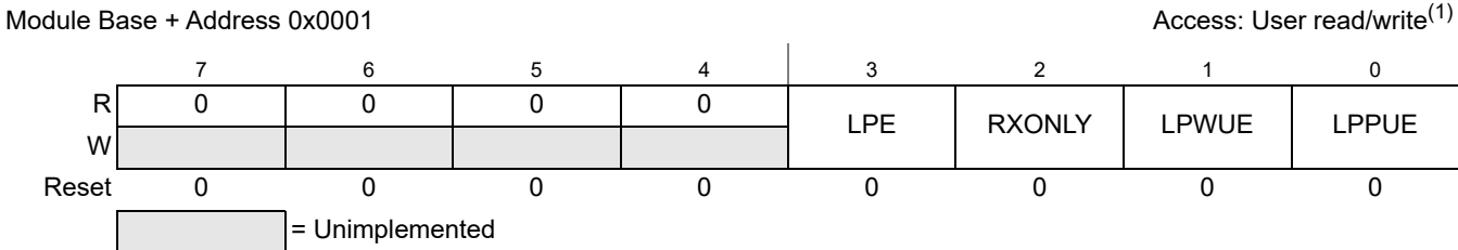
Figure 16-4. LIN Control Register (LPCR)
