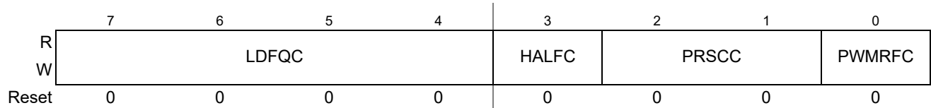
Figure 12-35. PMF Frequency Control C Register (PMFFQCC)
