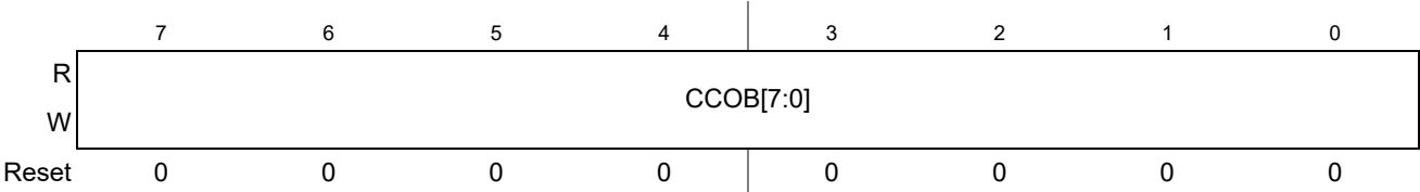
Figure 18-23. Flash Common Command Object 2 Low Register (FCCOB2LO)
