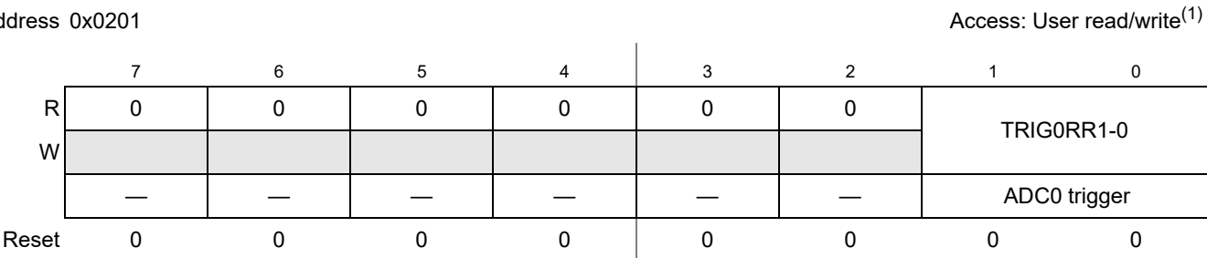
Figure 2-3. Module Routing Register 1 (MODRR1)
