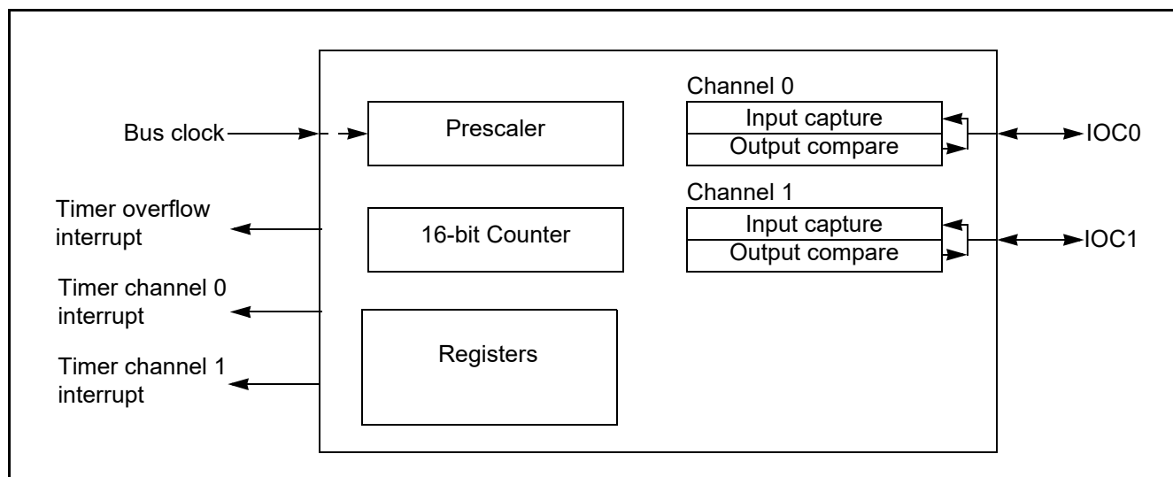
Figure 11-1. TIM16B2CV3 Block Diagram
