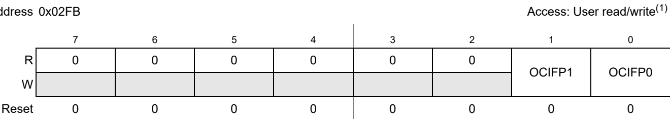
Figure 2-28. Port P Over-Current Interrupt Flag Register
