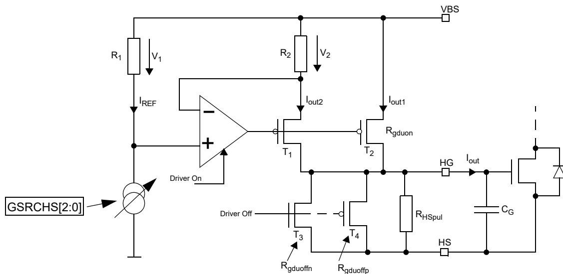
Figure 17-28. FET Pre-Driver Concept for High-Side Driver
