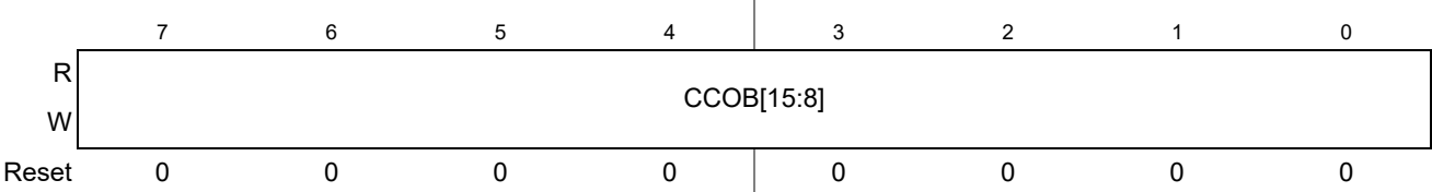
Figure 18-26. Flash Common Command Object 4 High Register (FCCOB4HI)
