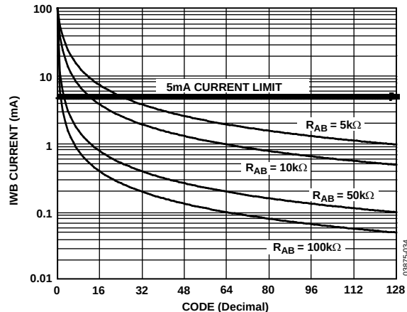
Figure 33. Maximum Operating Current
