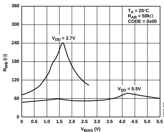
Figure 17. R_{WB} vs. V_{BIAS} vs. V_{DD}
