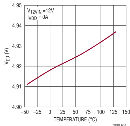
V_{\text{DD}} Regulator Output Voltage vs Temperature
