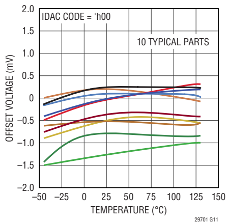
V_{\text{OUTn}} Offset Voltage vs Temperature
