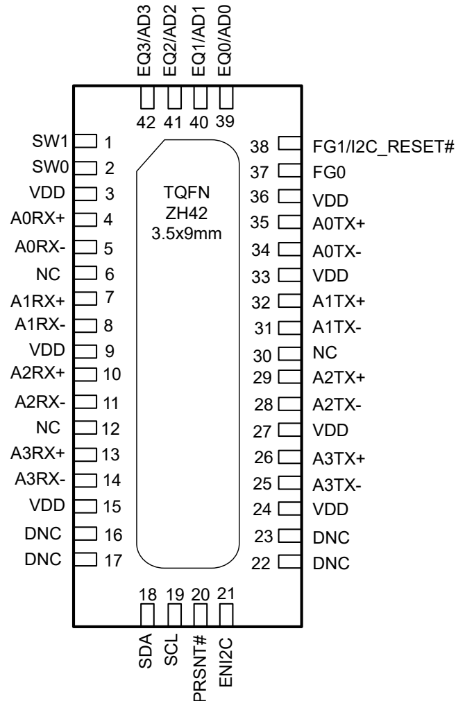
Figure 3-1 32/42-pin package pin-out
