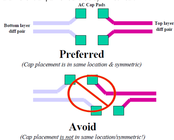
Figure 7-17 Layout Guidance of Series Component
