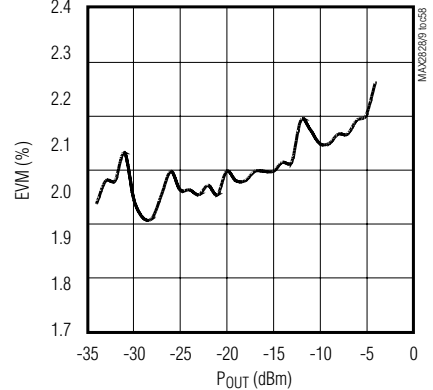
TX EVM vs. Pout
