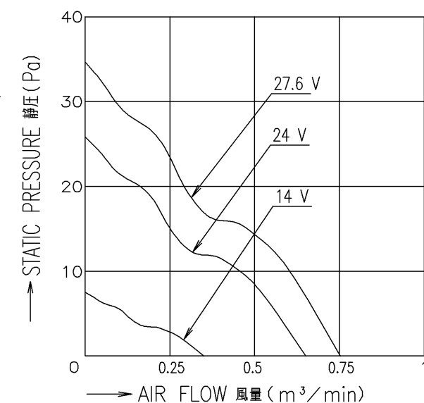
PERFORMANCE CURVES 風量-静圧特性例
