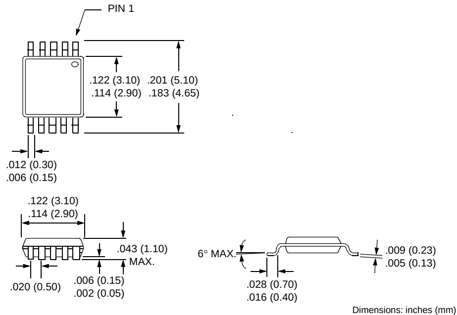
10-Pin MSOP
