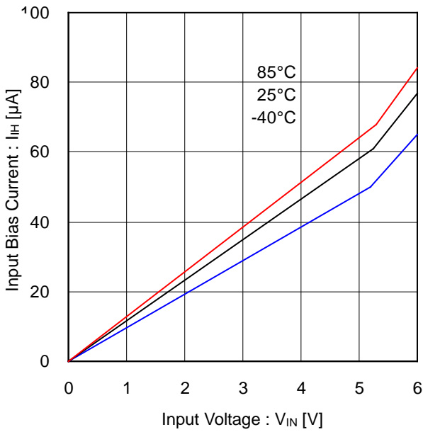
Figure 9. Input Bias Current vs Input Voltage
