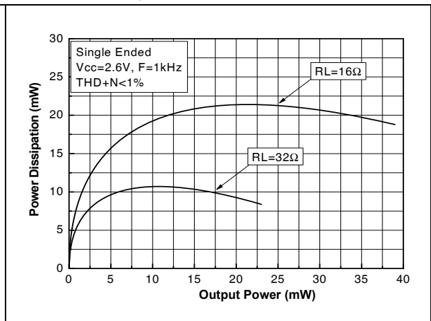
Figure 43. Power dissipation vs. output power, SE, V_{CC} = 2.6\text{ V}
