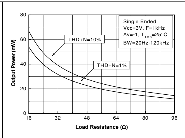
Figure 39. Output power vs. load resistance, SE, V_{CC} = 3\text{ V}
