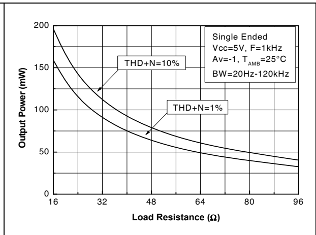
Figure 41. Output power vs. load resistance, SE, V_{CC} = 5\text{ V}
