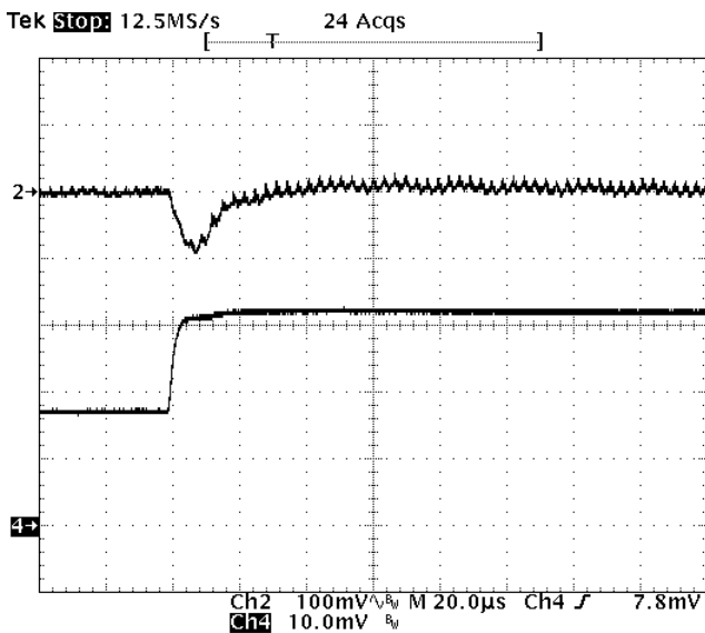
Fig-1.5V-6: Output voltage response for V_{out}=1.5V to positive load current step change from 8A to 16A with slew rate of 5A/us at V_{in}=12V . C_o=47\mu F \times 4 ceramic. Top trace: output voltage (100mV/div.) Bottom trace: load current (5A/div.) Time scale: 20us/div.
