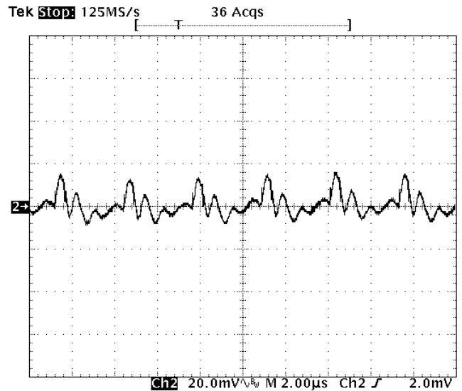
Fig-1.5V-5: Output voltage ripple (20mV/div.) for V_{out}=1.5V at full rated load current into a resistive load with external capacitance 47\mu F \times 4 ceramic + 1uF ceramic at V_{in}=12V . Time scale: 2us/div
