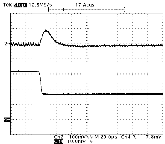
Fig-1.5V-7: Output voltage response for V_{out}=1.5V to negative load current step change from 16A to 8A with slew rate of -5A/us at V_{in}=12V . C_o=47\mu F \times 4 ceramic. Top trace: output voltage (100mV/div.) Bottom trace: load current (5A/div.) Time scale: 20us/div.
