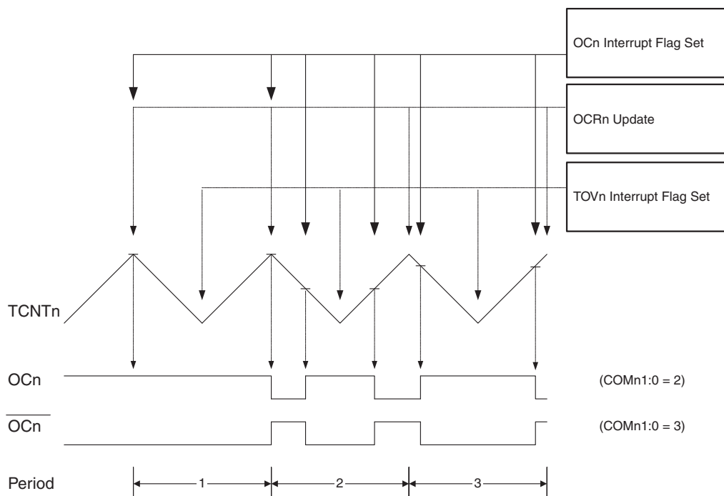
Figure 14-7. Phase Correct PWM Mode, Timing Diagram
