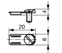
Screw-Adapter for Quick Connect-Terminals 6.3 x 0.8 mm
