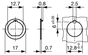
Transparent Cover 0853.0551 Reflow-Cover 0853.0571 Order No. OGN/OGN-SMD 0853.0551 * / 0853.0571 *
