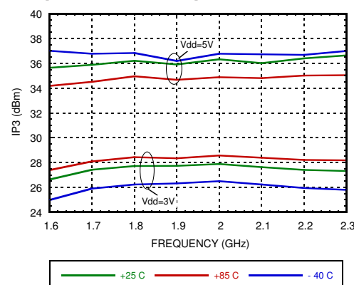
Output IP3 vs. Temperature [1] [2]
