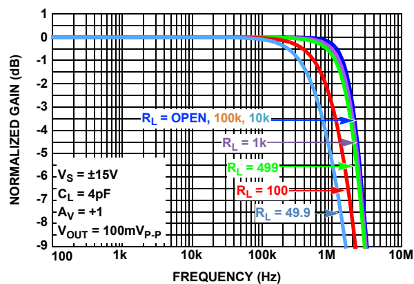
FIGURE 76. SIMULATED GAIN vs FREQUENCY vs R_L
