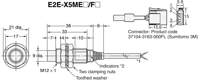
Diagram 10 E2E-X8MD□ Pre-wired e-CON Connector Models E2E-X5ME□/F□
