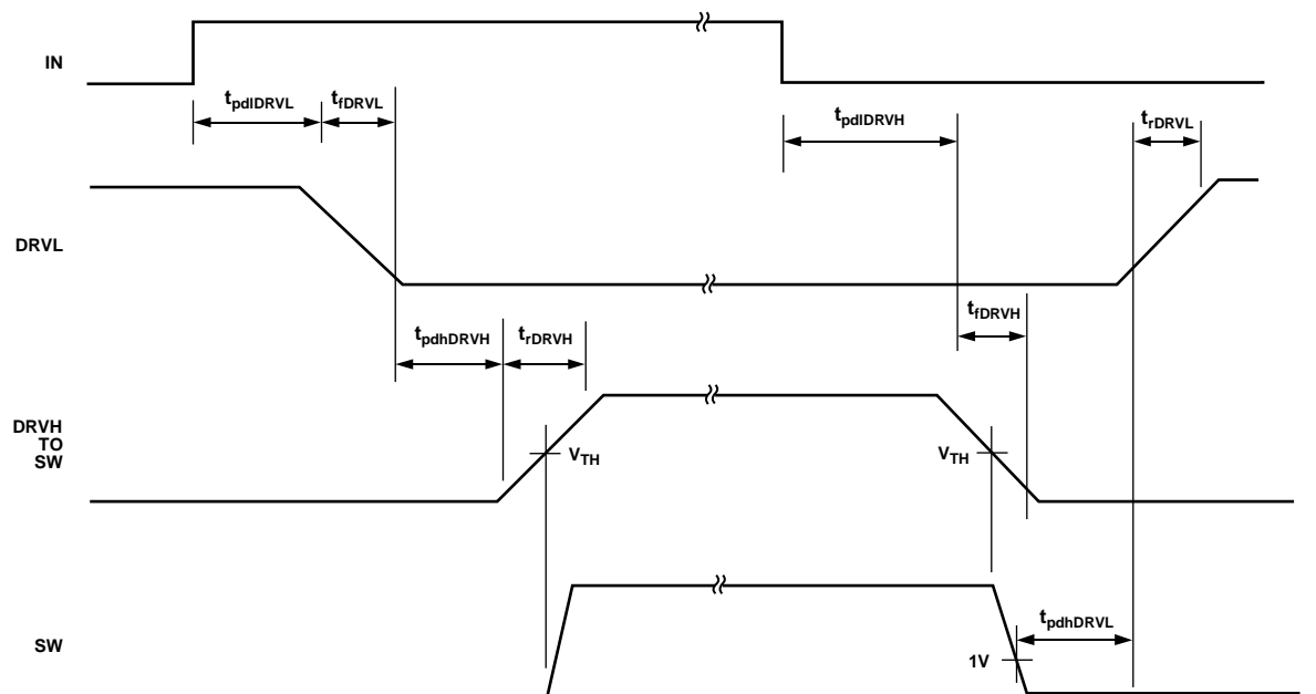
Figure 3. Timing Diagram
