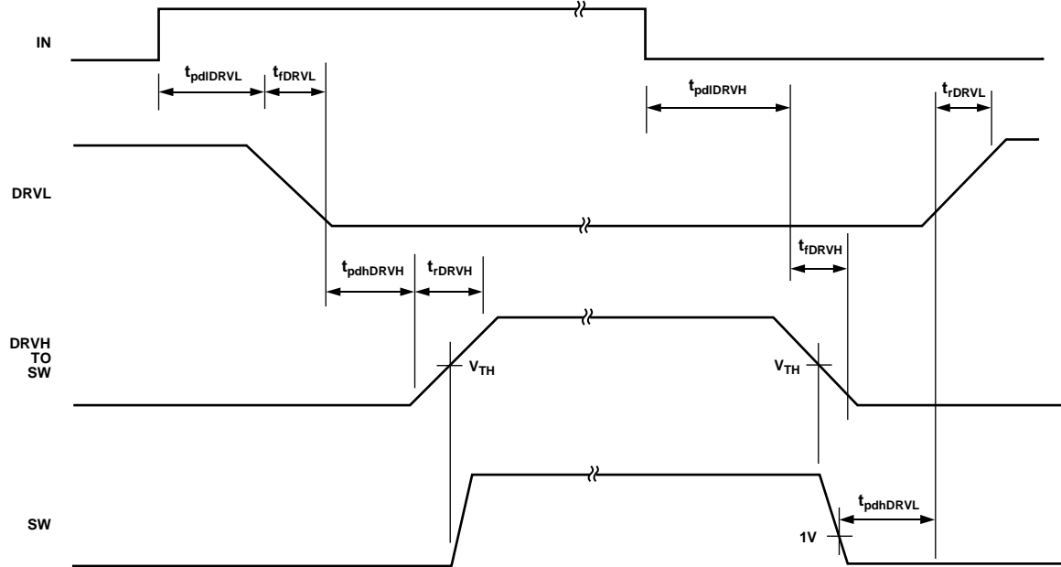
Figure 3. Timing Diagram
