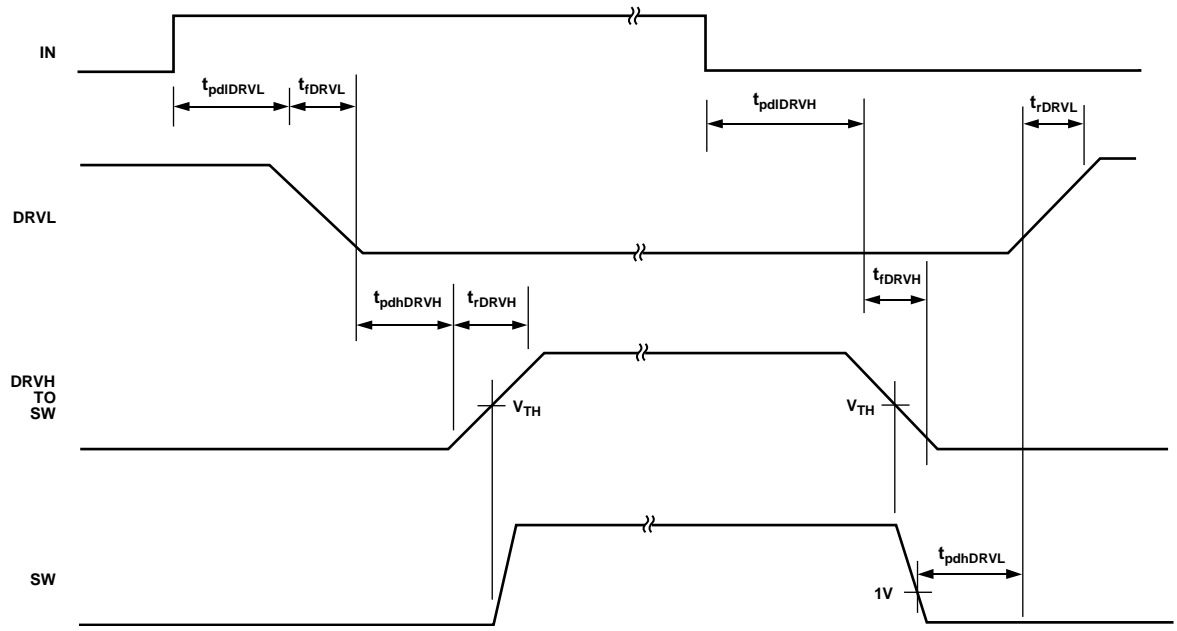
Figure 3. Timing Diagram
